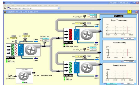
Mimic of clean air control system
